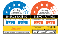
25 Class Model
